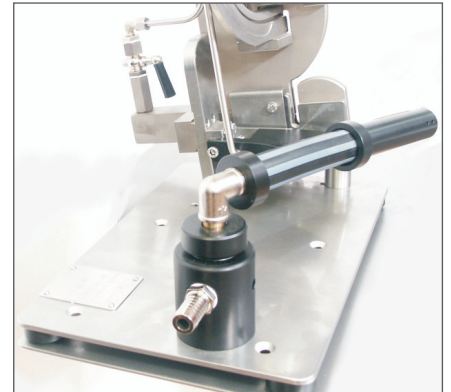
Tilttable suction tube for vacuum packaging
